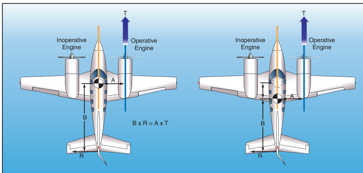
Figure 12-20. Effect of CG location on yaw.
